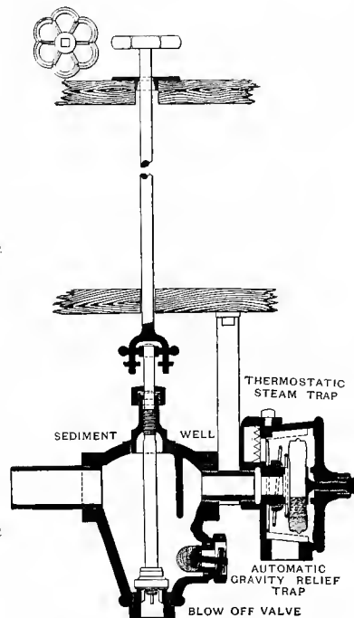
Fig. 3007 EXCELSIOR STEAM TRAP WITH SEDIMENT WELL, GRAVITY RELIEF TRAP AND SPECIAL BLOW-OFF VALVE.
